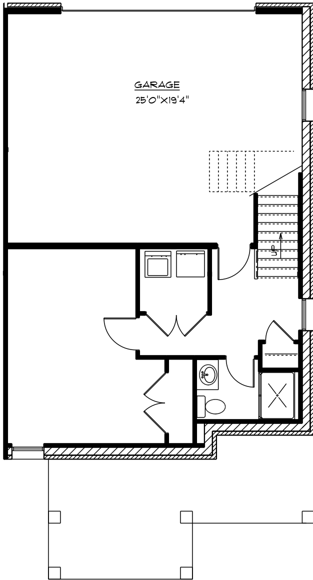
GROUND FLOOR PLAN UNIT C
