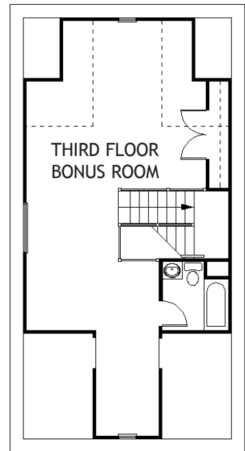
Charleston Third Floor Plan
