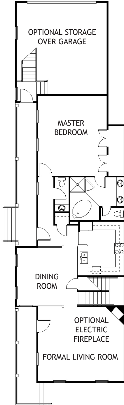
Charleston First Floor Plan
