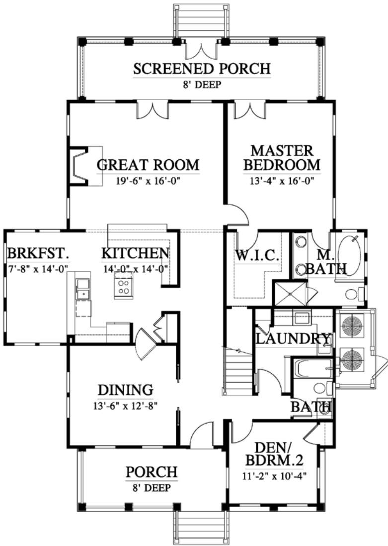
1ST FLOOR
